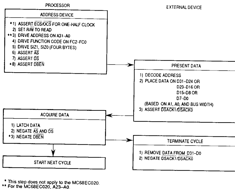
Figure 5-20. Byte Read Cycle Flowchart
