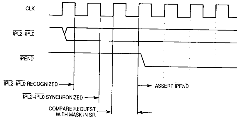
Figure 6-4. Assertion of \overline{IPEND} (MC68020 Only)
