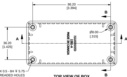
TOP VIEW OF BOX
