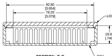
SECTION C-C SCALE 1 : 1
