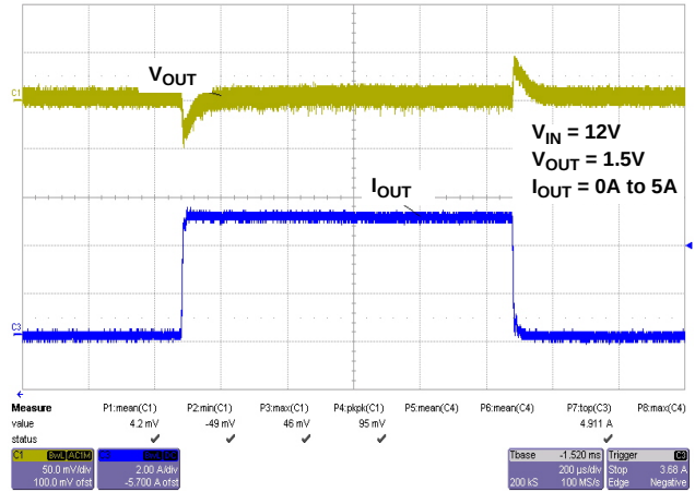
FIGURE 9. 1.5V TRANSIENT RESPONSE
