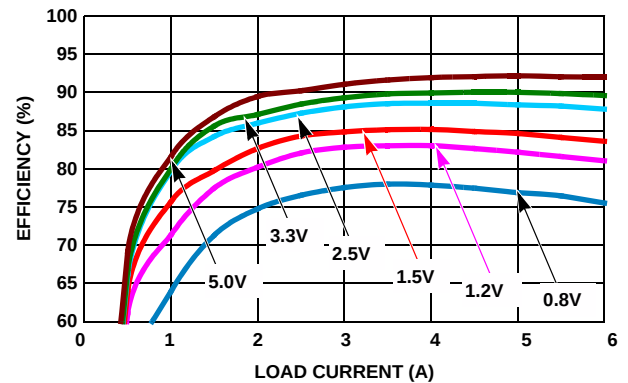
FIGURE 6. EFFICIENCY vs LOAD CURRENT ( 12\text{V}_{IN} )
