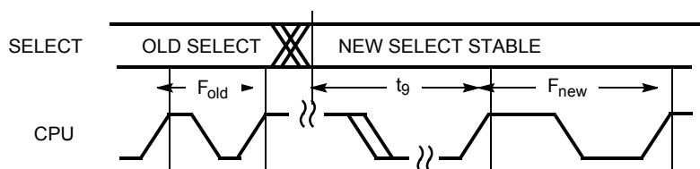
Figure 11. CPU Frequency Change
