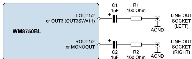
The DC blocking capacitors and the load resistance together determine the lower cut-off frequency, f_c . Assuming a 10 kOhm load and C_1, C_2 = 1\mu F :
