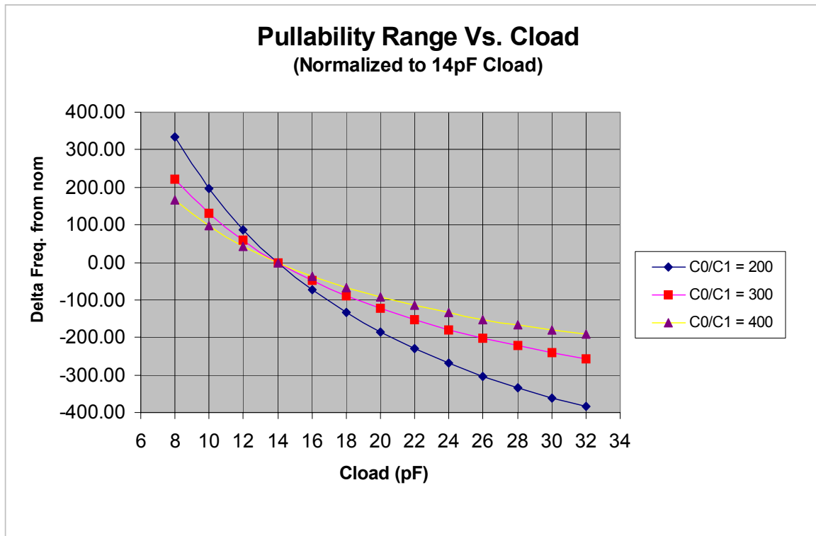
Figure 8. Frequency vs. Load Behavior for Example XTAL
