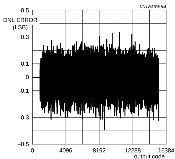
Fig 16. DNL error as a function of output code
