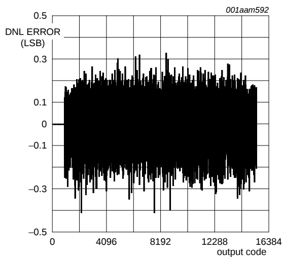
Fig 18. DNL error as a function of output code
