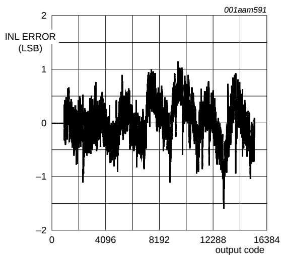
Fig 17. INL error as a function of output code
