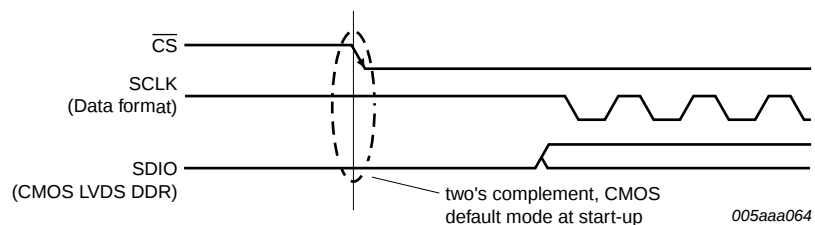
Fig 38. Default mode at start-up: SCLK HIGH = two's complement; SDIO LOW = CMOS
