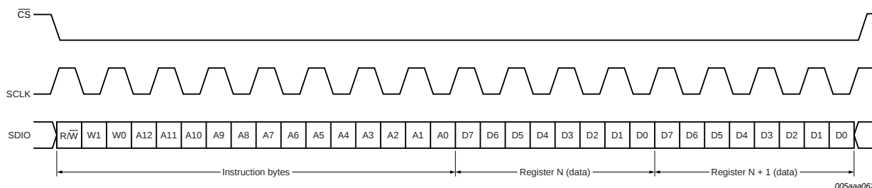
Fig 36. SPI mode timing
