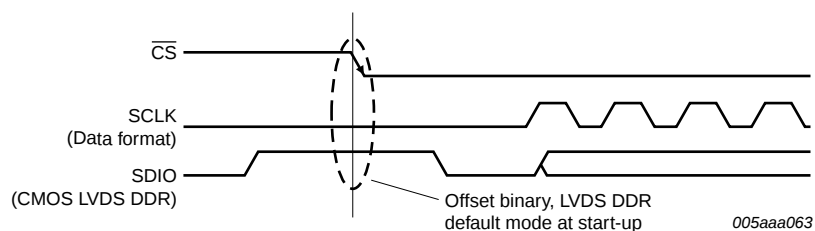
Fig 37. Default mode at start-up: SCLK LOW = offset binary; SDIO HIGH = LVDS DDR
