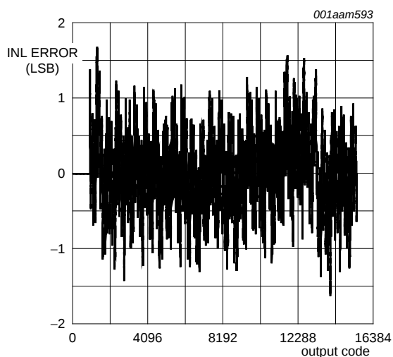
Fig 15. INL error as a function of output code
