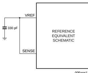
Fig 28. Internal reference via SPI, 1 V (p-p) to 2 V (p-p) full-scale
