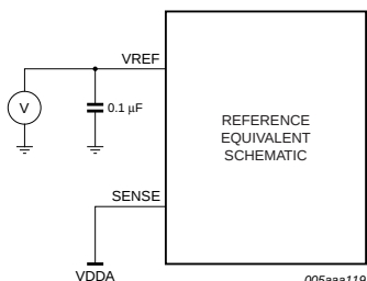
Fig 27. External reference, 1 V (p-p) to 2 V (p-p) full-scale
