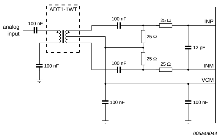
Fig 22. Single transformer configuration suitable for baseband applications
