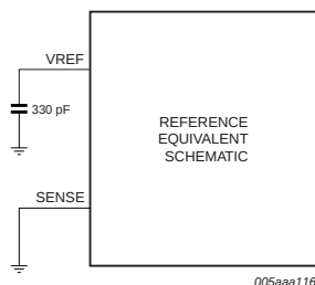
Fig 25. Internal reference, 2 V (p-p) full-scale
