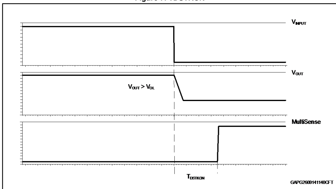
Figure 7: TDSTKON
