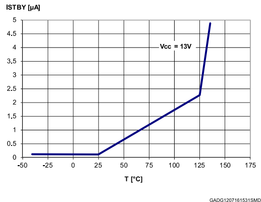
Figure 9: Standby current
