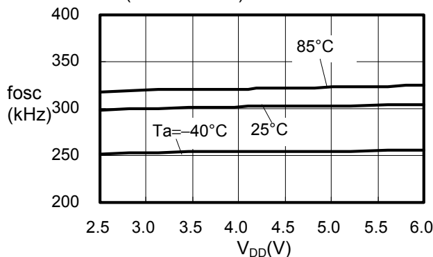
S-8340C33A(fosc:300 kHz)
