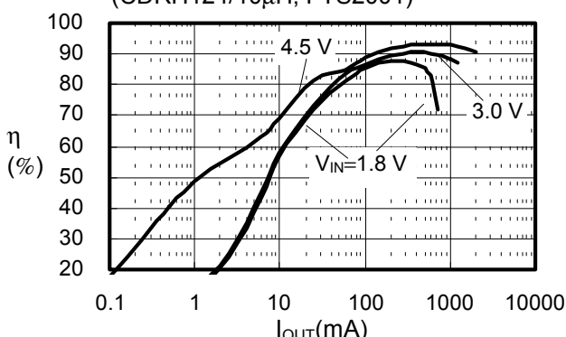
(24) S-8341C50AFT
