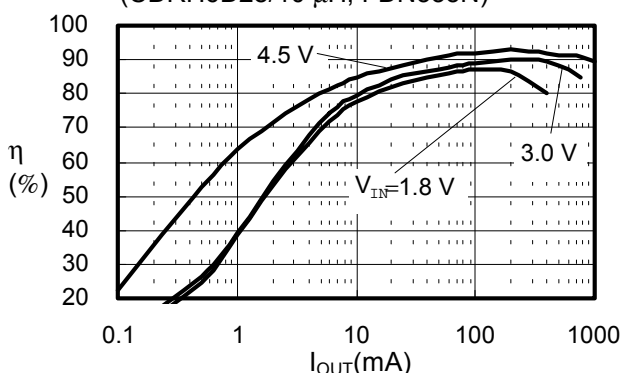
(23) S-8341C50AFT
