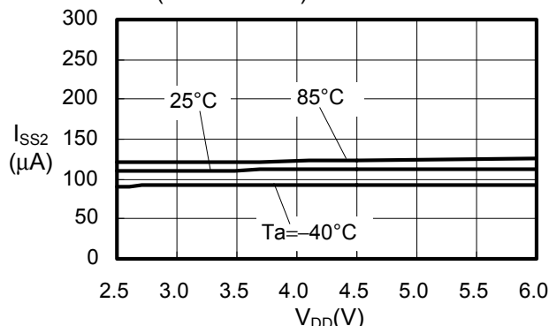
S-8340C33A(fosc:300 kHz)
