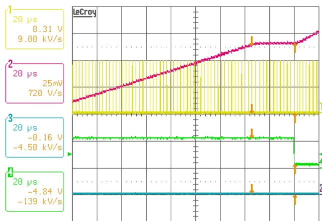
FIGURE 31. CPU MODE CLK_EN# DELAY, V IN = 19V, I O = 0A, VID = 1.2V, Ch1: PHASE1, Ch2: V O , Ch4: CLK_EN#
