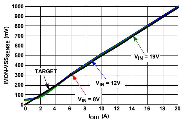
FIGURE 39. IMON, V_{ID} = 1.2375
