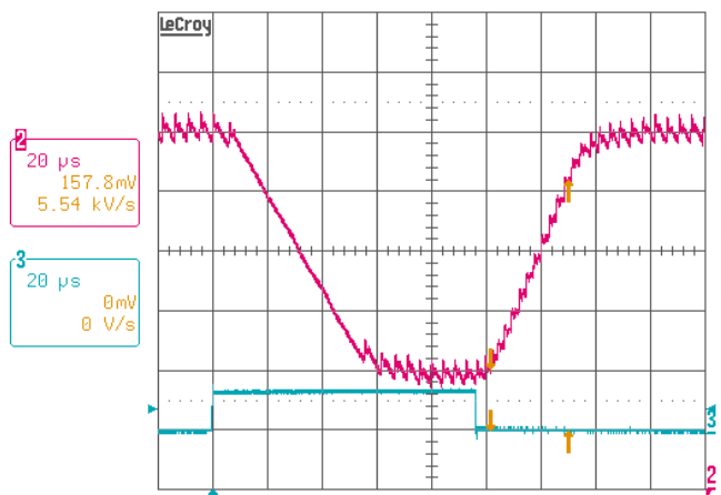
FIGURE 46. CPU MODE VID TRANSITION, DPRSLPVR = 1, I O = 2A, VID = 1.2375V/1.0375V, Ch2: V O , Ch3: VID4
