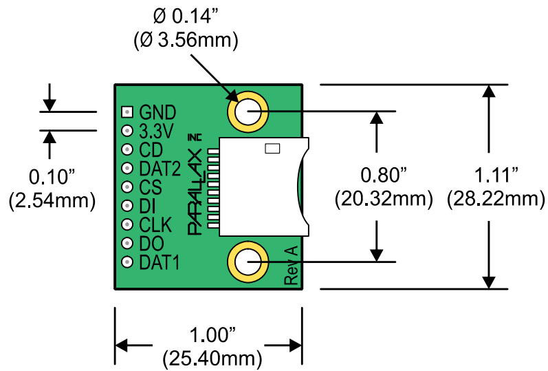
Figure 2: Module Dimensions
