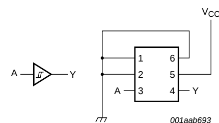
Fig 10. Buffer
