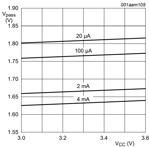
Fig. 8. Pass voltage versus supply voltage; T_{amb} = 0\text{ °C} (typical)
