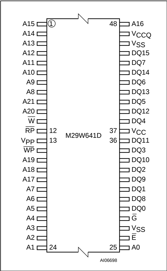
Figure 3. TSOP Connections
