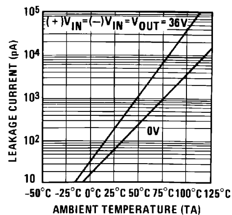
Leakage Current
