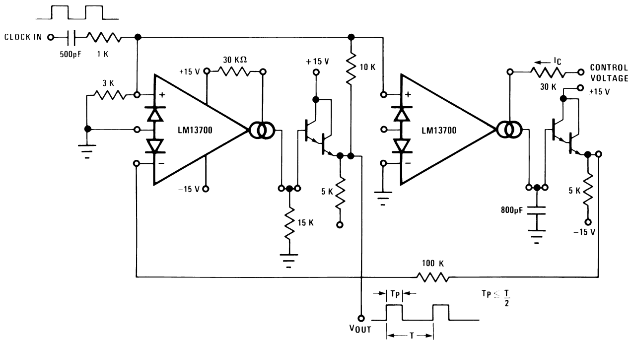
FIGURE 29. Pulse Width Modulator
