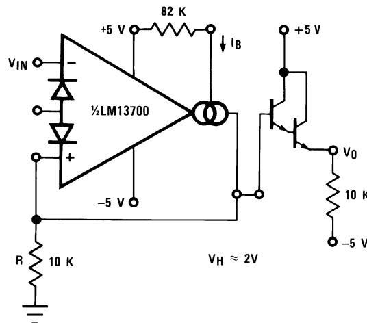
FIGURE 22. Schmitt Trigger
