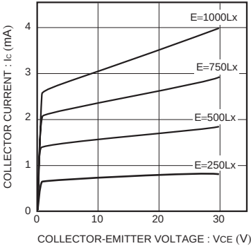
Fig.2 Output characteristics
