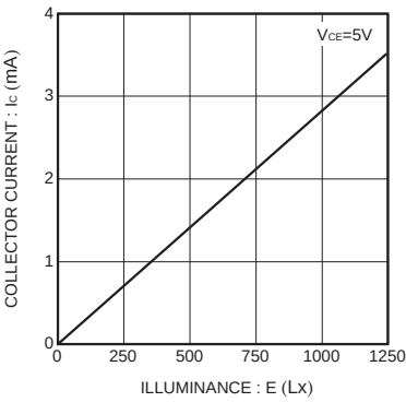
Fig.1 Collector current-Illuminance
