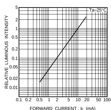
Fig.17 Luminous intensity vs. forward current
