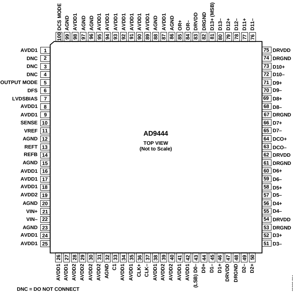
Figure 4. 100-Lead TQFP/EP Pin Configuration in LVDS Mode
