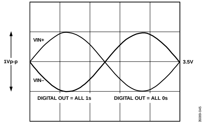
Figure 42. Differential Analog Input Range for VREF = 1 V
