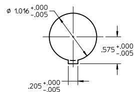
RECOMMENDED MOUNTING CUTOUT SCALE: 1:1
