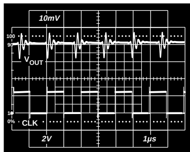
Figure 10. Clock Feedthrough vs. Time
