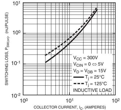
SWITCHING LOSS (ON) VS. COLLECTOR CURRENT (TYPICAL)
