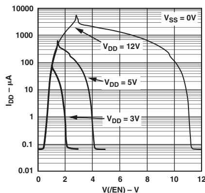
TPC 15. V_{DD} Current vs. Logic Level
