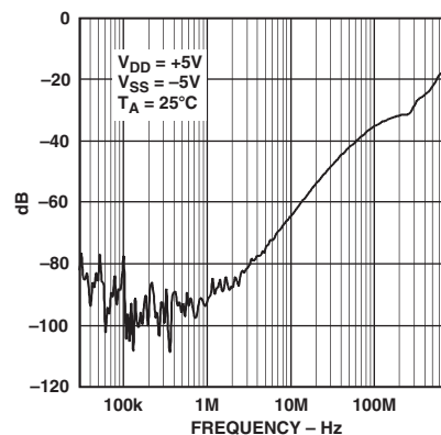
TPC 12. OFF Isolation vs. Frequency
