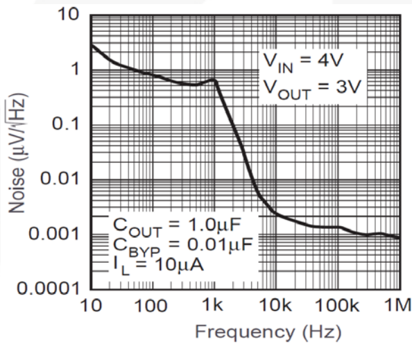
Figure 11. Noise Performance
