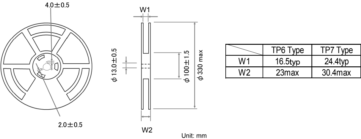
Figure 4 Reel Forms
