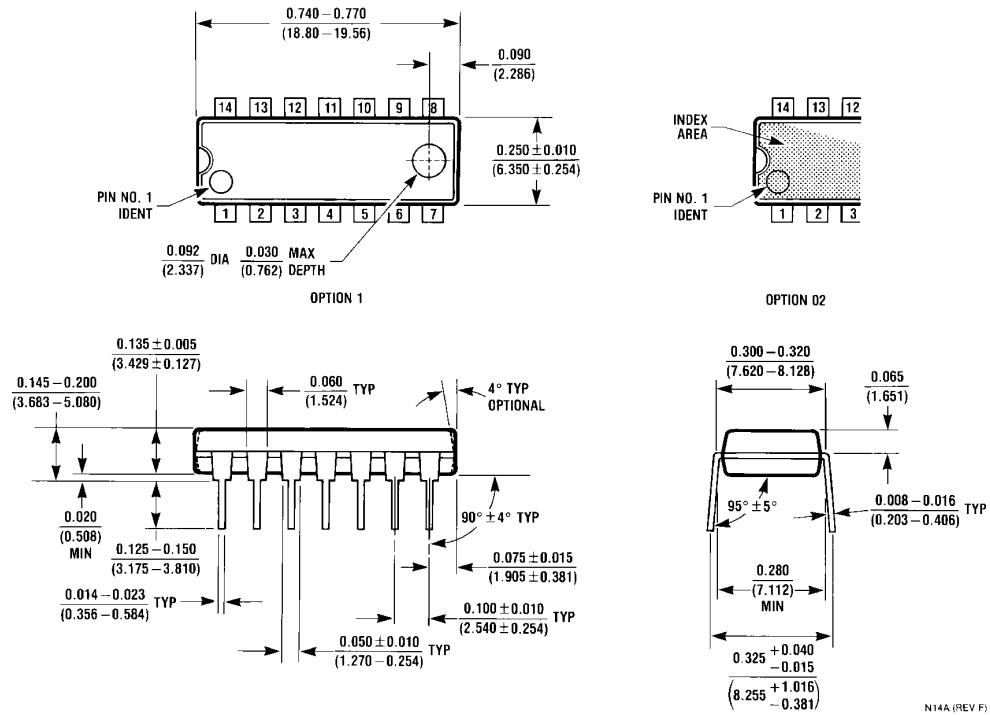
Molded Dual-In-Line Package (N) Order Number LM1815N NS Package Number N14A
