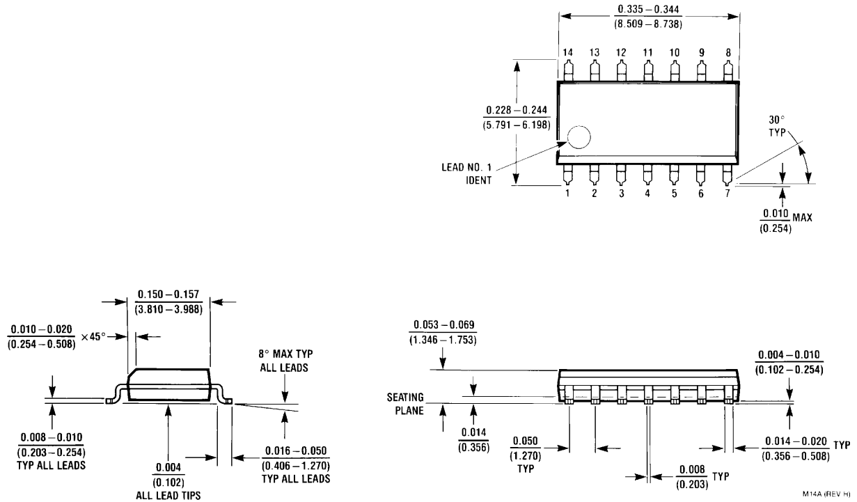
14-Lead Small Outline Circuit (M) Order Number LM1815M NS Package Number M14A
