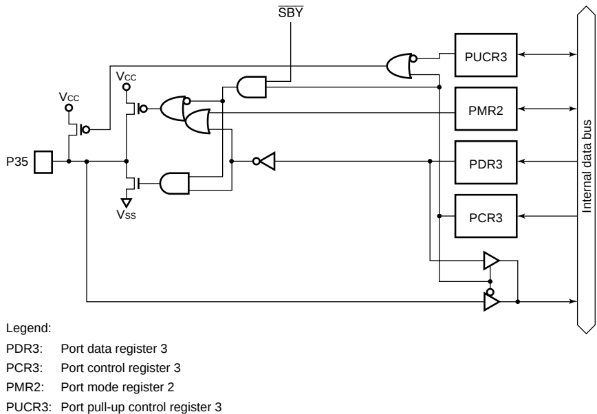
Figure B.1(b) Port 3 Block Diagram (Pin P35)
