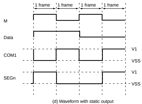
Figure 13.8 Output Waveforms for Each Duty Cycle (B Waveform)
