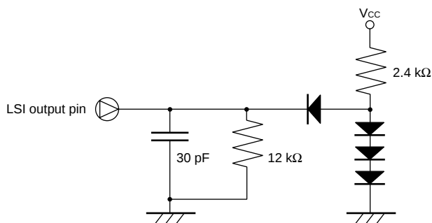
Figure 17.6 Output Load Circuit
