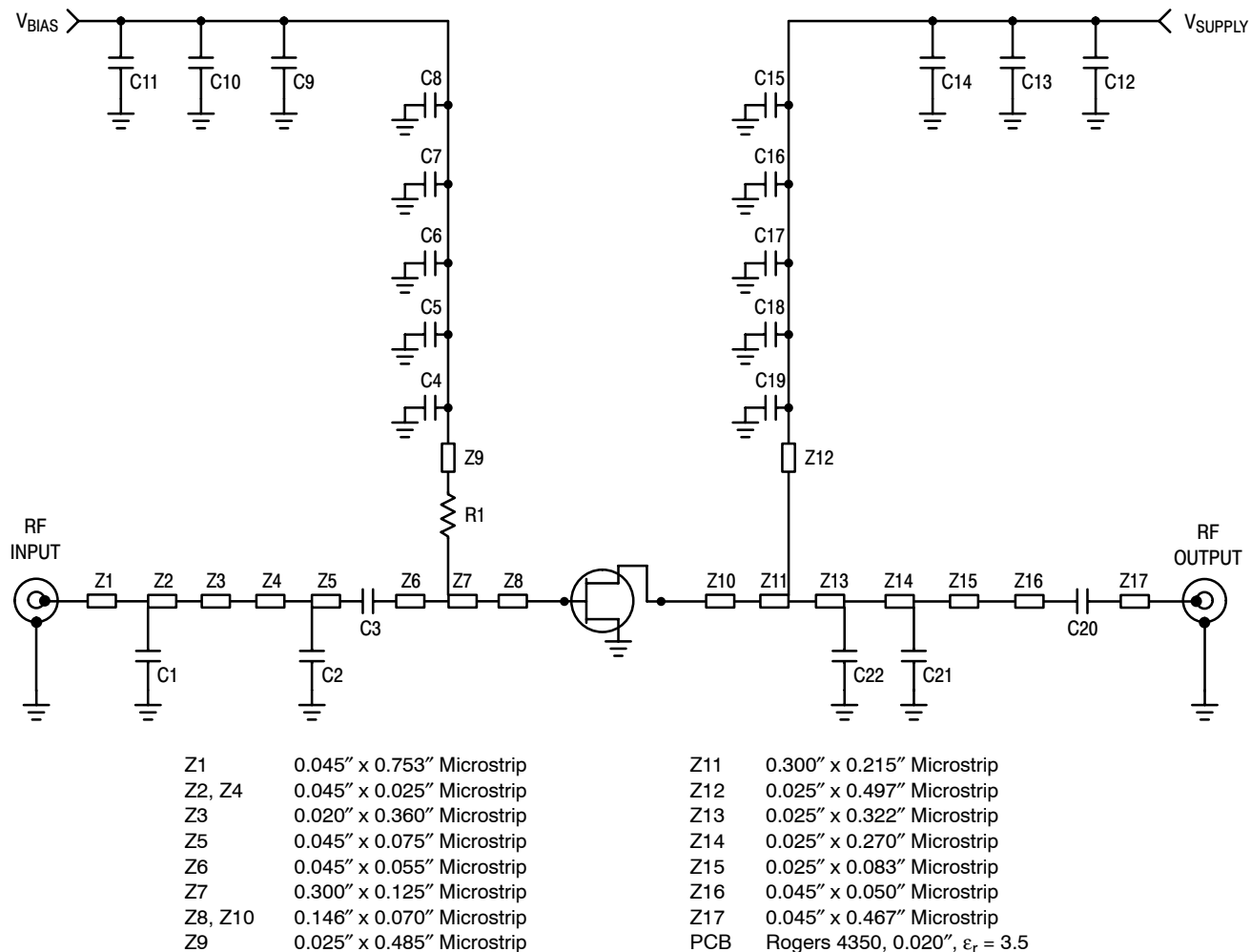
Figure 1. MRFG35003N6A Test Circuit Schematic
