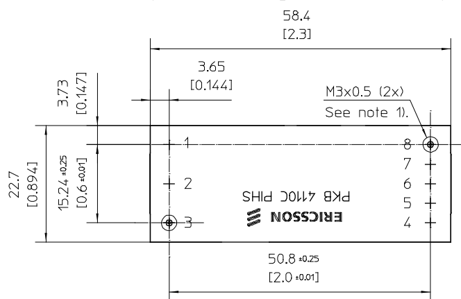
RECOMMENDED FOOTPRINT
