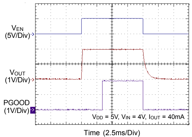
PGOOD Response
