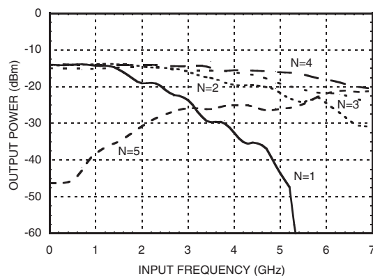
5th Harmonic, N = 1 through 5
