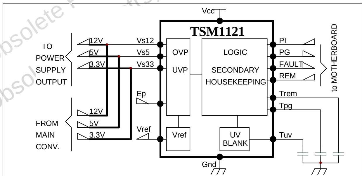
Fig. 2: Internal Schematic
