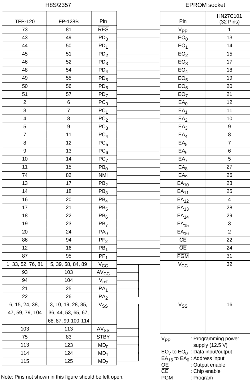
Figure 19-2 Wiring of 120/128B-Pin Socket Adapter
