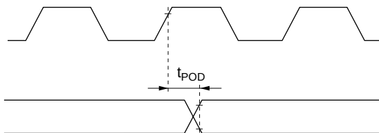
Figure 22-23 PPG Output Timing
