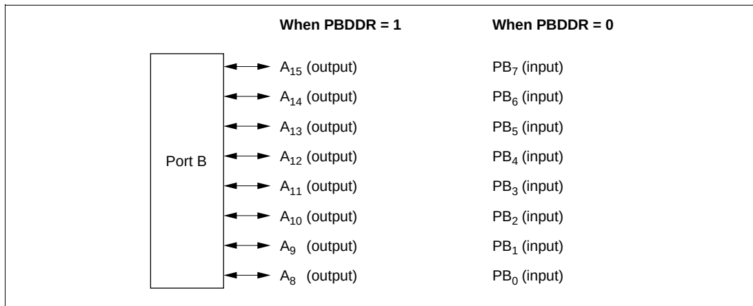
Figure 9-13 Port B Pin Functions (Modes 6)
