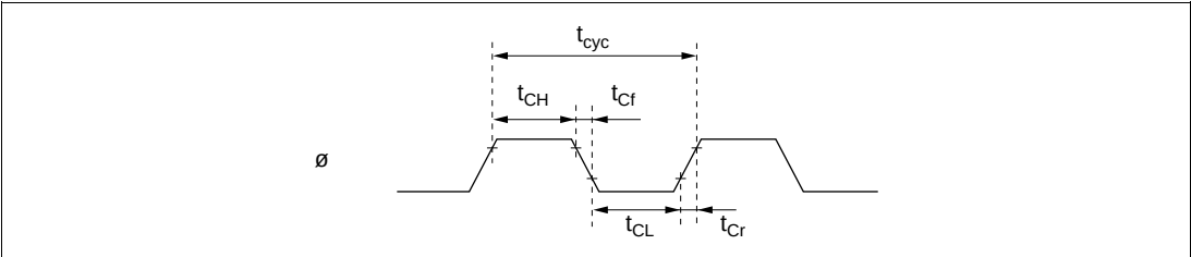
Figure 22-36 System Clock Timing
