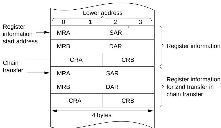
Figure 8-5 Location of Register Information in Address Space
