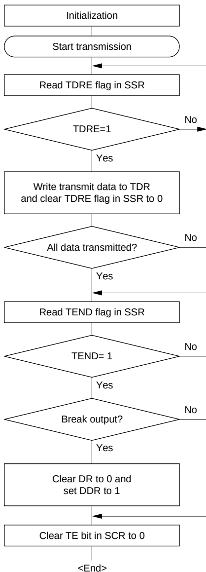
Figure 14-5 Sample Serial Transmission Flowchart
