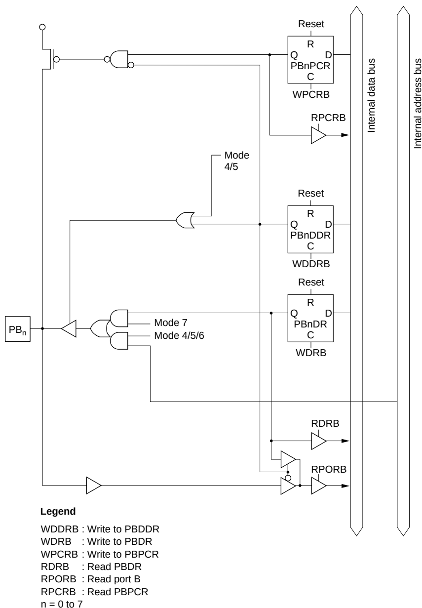
Figure C-8 Port B Block Diagram (Pin PB 0 to PB 7 )
