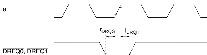
Figure 22-53 DMAC \overline{DREQ} Input Timing
