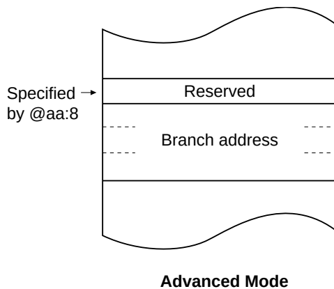
Figure 2-10 Branch Address Specification in Memory Indirect Mode
