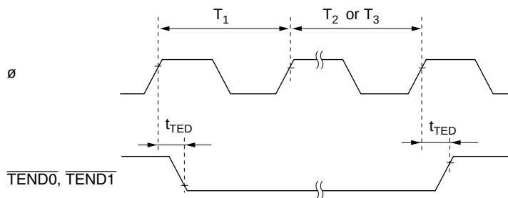
Figure 22-84 DMAC \overline{TEND} Output Timing
