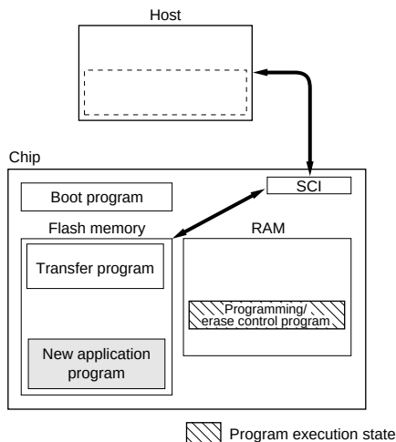
Figure 19-39 User Program Mode (Example)
