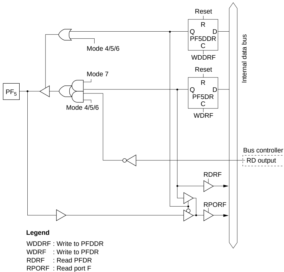
Figure C-12 (f) Port F Block Diagram (Pin PF 5 )
