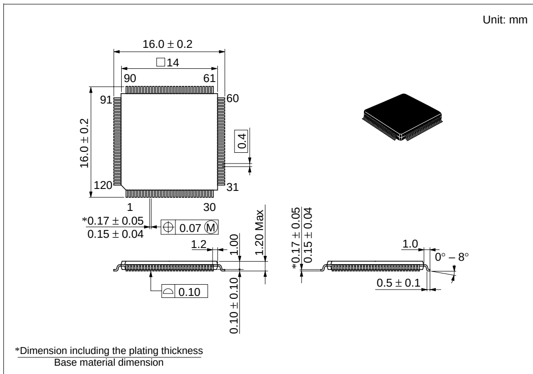
Figure H-1 TFP-120 Package Dimension
