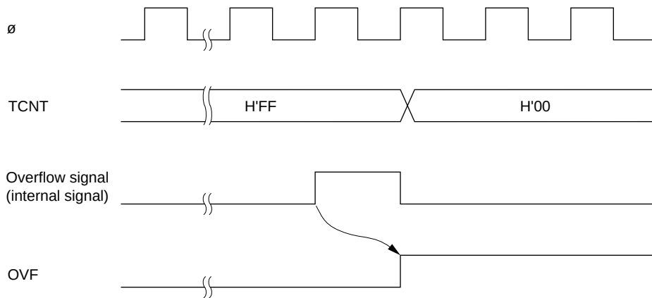
Figure 13-6 Timing of Setting of OVF
