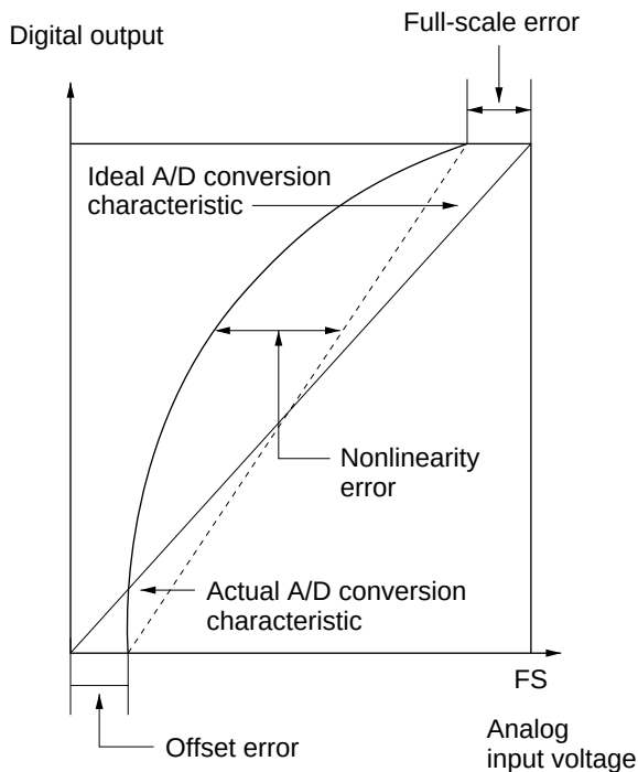
Figure 16-9 A/D Conversion Precision Definitions (2)
