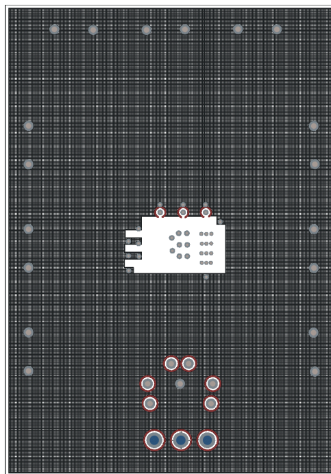
(b) DEM-OPA-SSOP-3C Mid Layer 1
