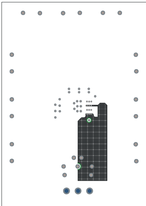
(c) DEM-OPA-SSOP-3C Mid Layer 2
