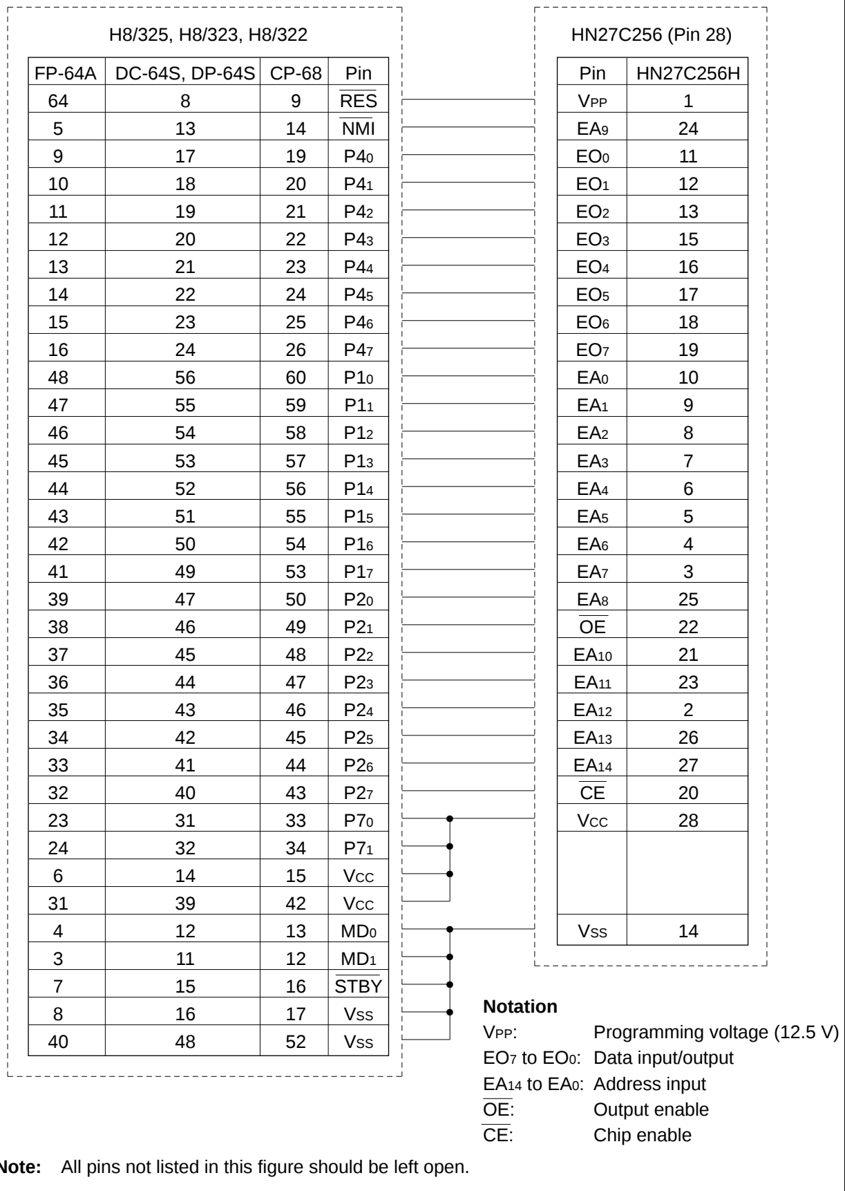
Figure 11-3. Socket Adapter Pin Assignments
