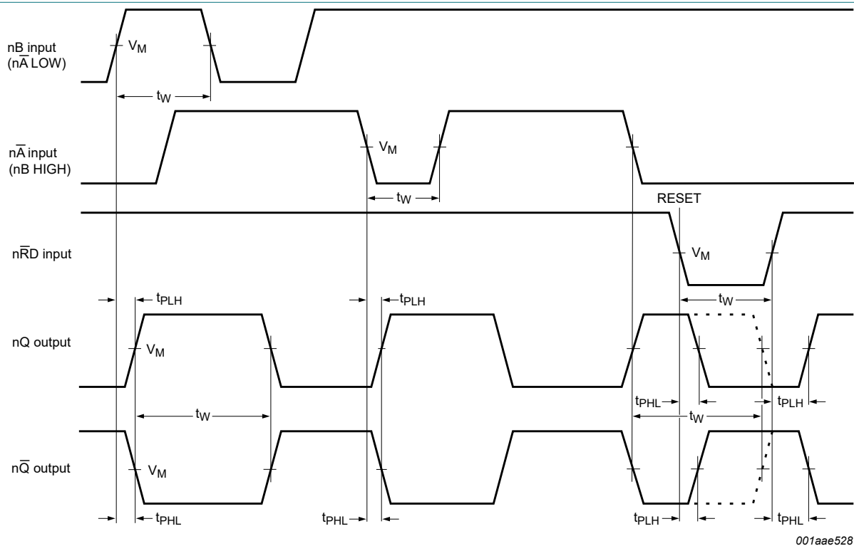
Fig. 5. Propagation delays from inputs ( n\bar{A} , nB , n\bar{RD} ) to outputs ( nQ , n\bar{Q} )
