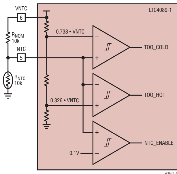
Figure 4. NTC Circuit
