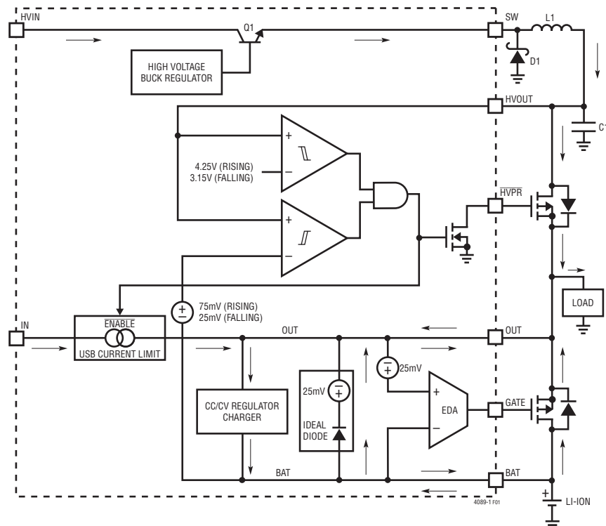
Figure 1. Simplified PowerPath Block Diagram
