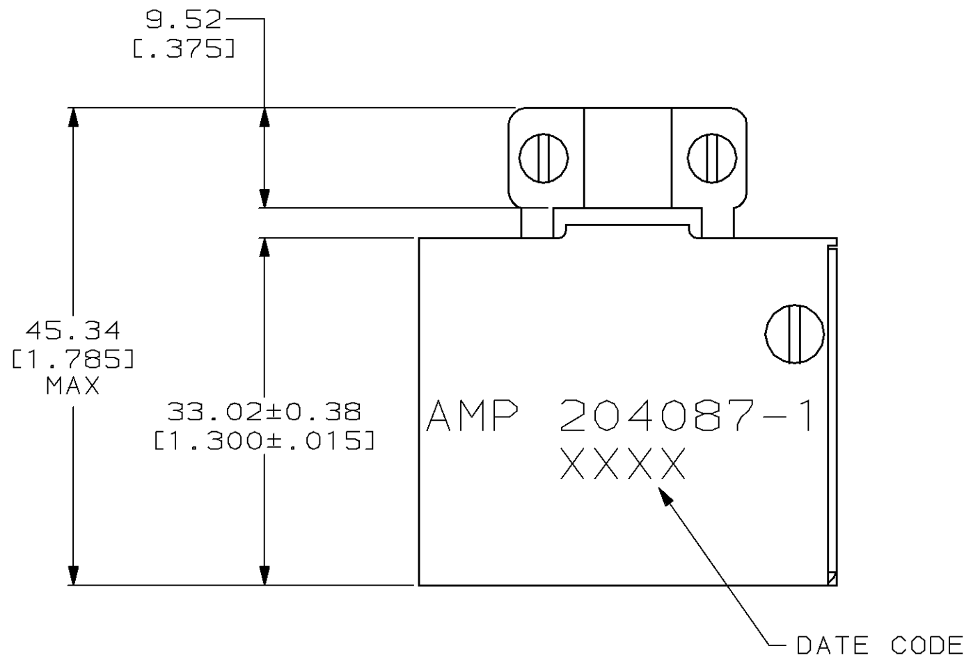
ASSEMBLED VIEW
