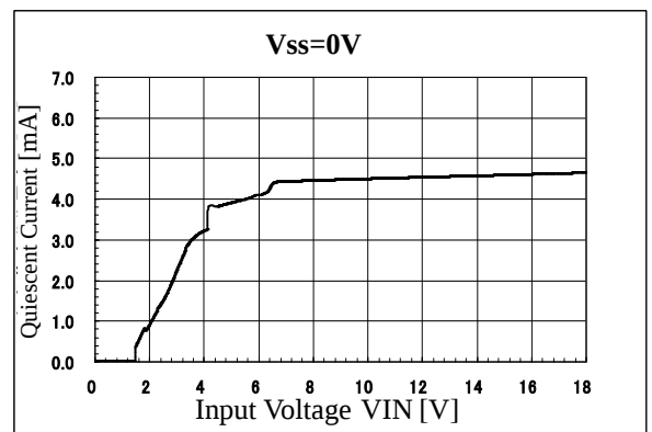
Quiescent Current
