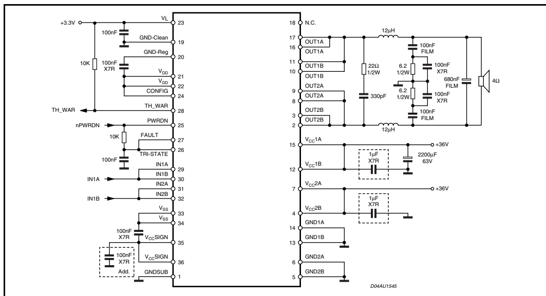
Figure 6. Typical single BTL configuration to obtain 350 W @ THD 10 %, R_L = 4 \Omega , V_{CC} = 54 \text{ V} (a)
