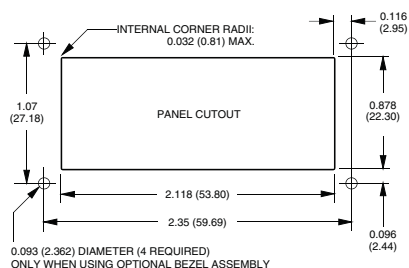
RECOMMENDED DRILL AND PANEL CUTOUT DIMENSIONS
