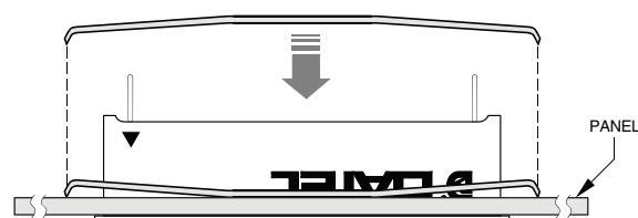
RETAINING CLIP INSTALLATION
