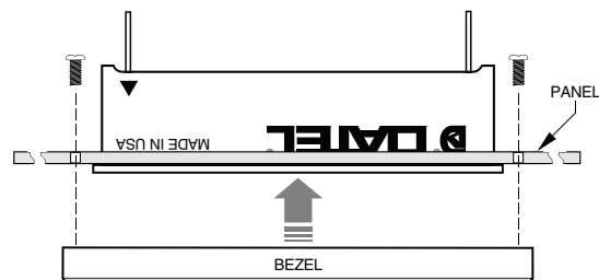
RETAINING CLIP INSTALLATION
