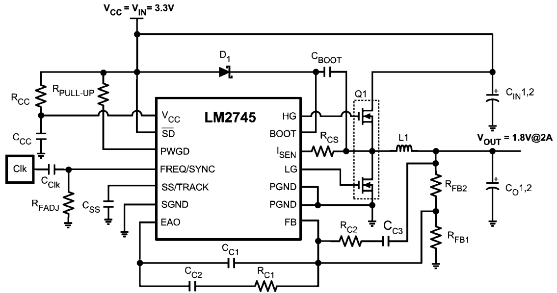
FIGURE 17. 3.3V to 1.8V @ 2A, f_{sw} = 300 \text{ kHz}
