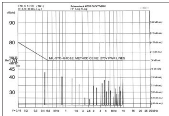
Figure 1– M-FIAM3 and Model V300A48M500AL DC-DC converter operating at 180Vdc, 130W.
