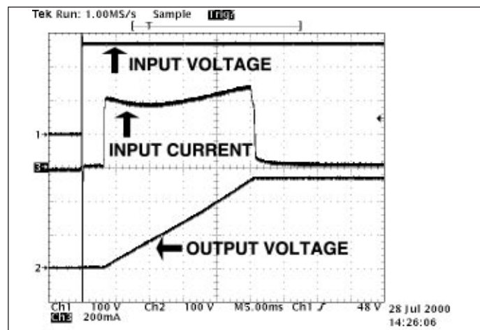
Figure 3– Inrush Limiting: Inrush current with 33μF external capacitance.
