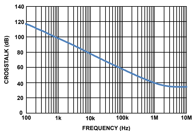
FIGURE 29. CROSSTALK ( V_{\pm} = \pm 15V , R_L = 1k\Omega , +25^{\circ}\text{C} )
