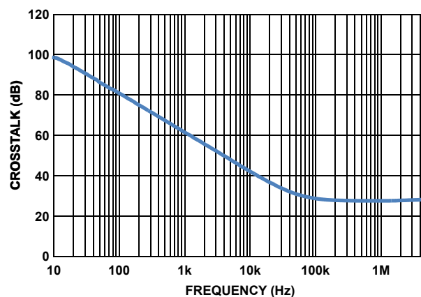
FIGURE 30. CROSSTALK ( V_{\pm} = \pm 15V , R_L = \text{OPEN} , +25^{\circ}\text{C} )
