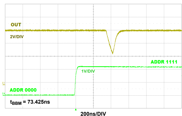
FIGURE 25. TYPICAL BREAK-BEFORE-MAKE DELAY ( V_{\pm} = 15V , +25^{\circ}\text{C} )
