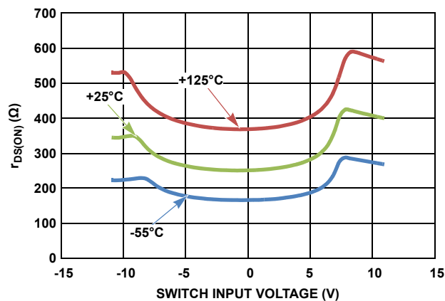
FIGURE 16. r_{DS(ON)} vs V_{CM} ( V_{\pm} = 10.8V )
