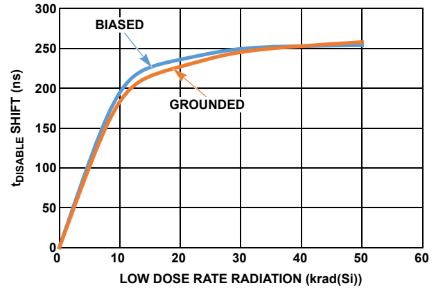
FIGURE 43. t_{\text{DISABLE}} SHIFT vs LDR RADIATION
