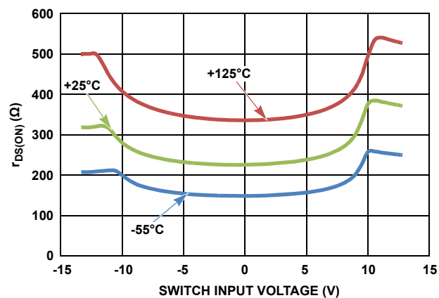
FIGURE 18. r_{DS(ON)} vs V_{CM} ( V_{\pm} = 13.2V )
