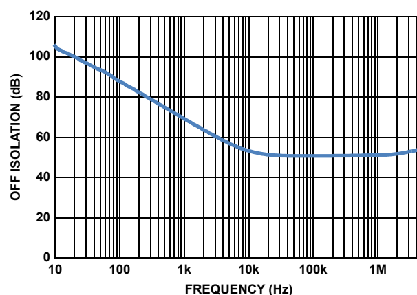
FIGURE 28. OFF ISOLATION ( V_{\pm} = \pm 15V , R_L = \text{OPEN} , +25^{\circ}\text{C} )
