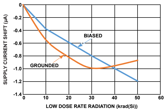
FIGURE 33. I_{EE} SUPPLY CURRENT SHIFT vs LDR RADIATION
