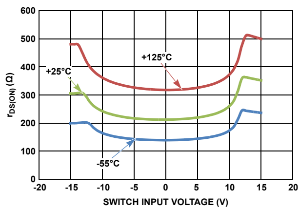
FIGURE 14. r_{DS(ON)} vs V_{CM} ( V_{\pm} = 15.0V )
