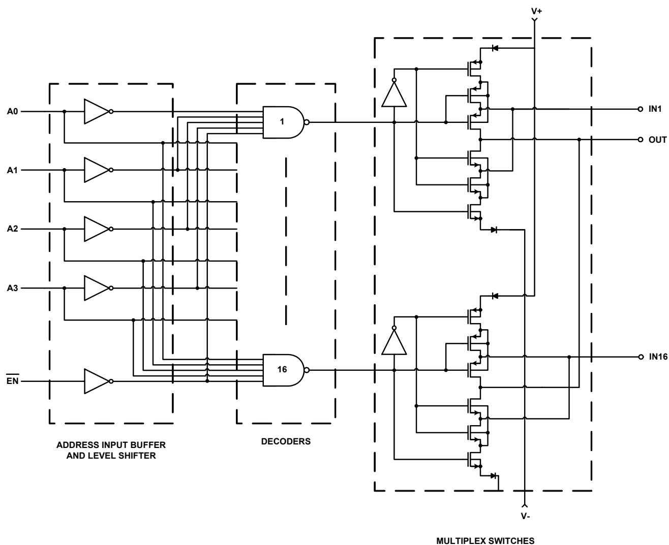
FIGURE 4. BLOCK DIAGRAM
