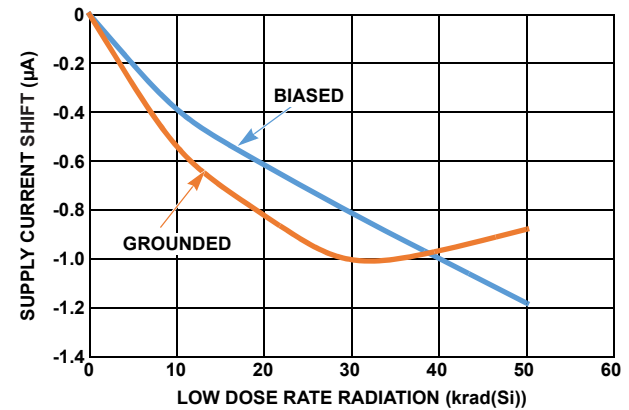
FIGURE 45. I_{EE} SUPPLY CURRENT SHIFT vs LDR RADIATION
