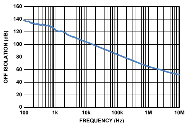
FIGURE 27. OFF ISOLATION ( V_{\pm} = \pm 15V , R_L = 1k\Omega , +25^{\circ}\text{C} )
