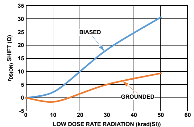
FIGURE 47. r_{DS(ON)} SHIFT ( V_{IN} = V^+ ) vs LDR RADIATION
