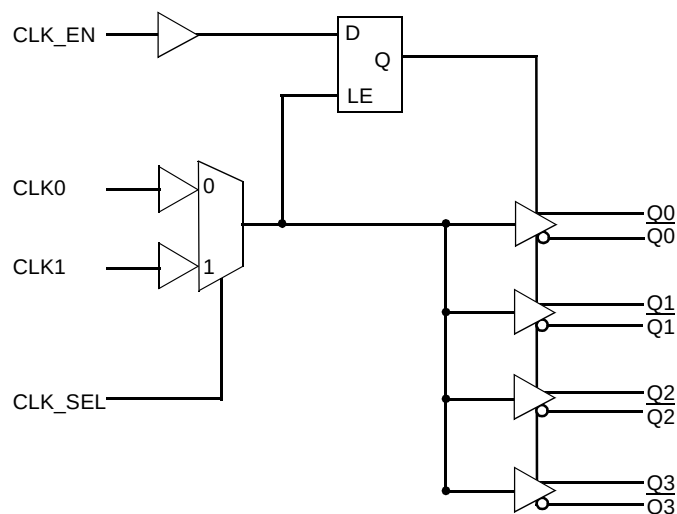
Figure 1. Logic Diagram
