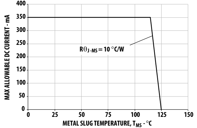
Figure 6. Maximum Forward Current vs. Metal Slug Temperature for AllnGaP Derated based on T_{JMAX} = 125\text{ °C} , R_{\theta J-MS} = 10\text{ °C/W}
