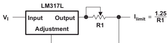
Figure 7-5. Precision Current-Limiter Circuit
