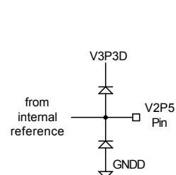
V2P5 Equivalent Circuit
