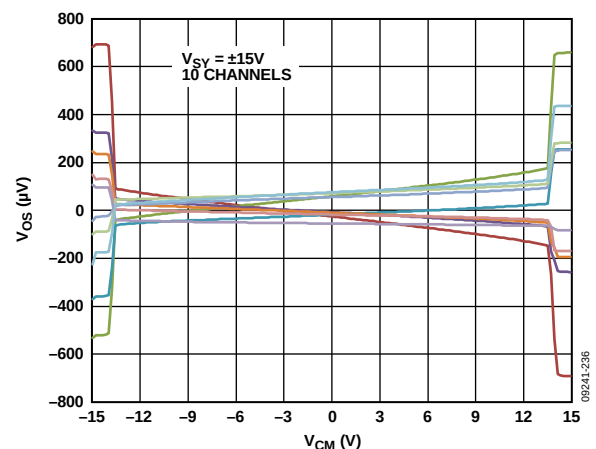
Figure 36. Input Offset Voltage ( V_{OS} ) vs. Common-Mode Voltage ( V_{CM} )
