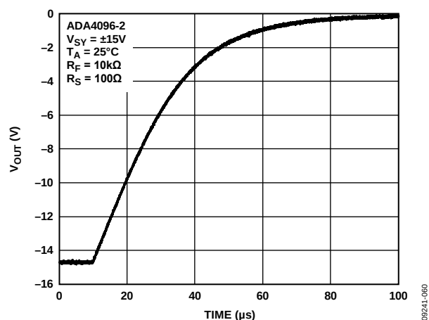
Figure 46. Negative Overload Recovery
