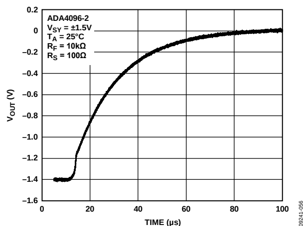
Figure 20. Negative Overload Recovery
