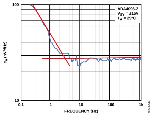
Figure 51. Voltage Noise Density ( e_n ) vs. Frequency
