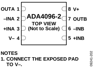
Figure 5. 8-Lead LFCSP (CP-8-10), ADA4096-2
