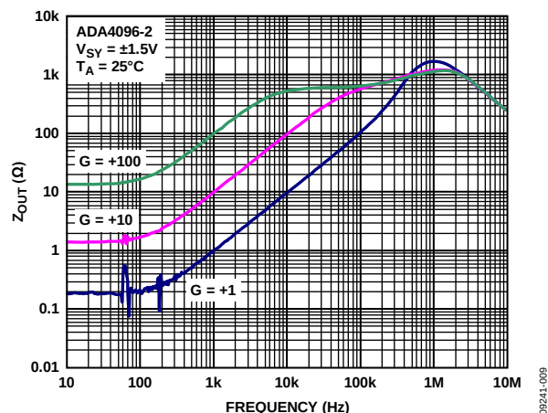
Figure 15. Output Impedance ( Z_{OUT} ) vs. Frequency
