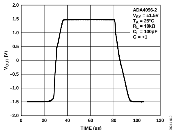
Figure 17. Large Signal Transient Response
