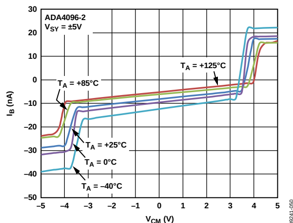
Figure 24. Input Bias Current ( I_B ) vs. V_{CM} for Various Temperatures
