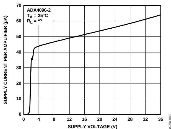
Figure 50. Supply Current per Amplifier vs. Supply Voltage
