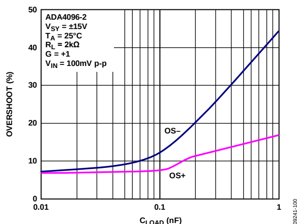
Figure 52. Overshoot vs. Load Capacitance ( C_{LOAD} )
