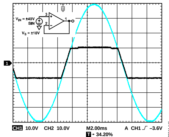
Figure 3. No Phase Reversal
