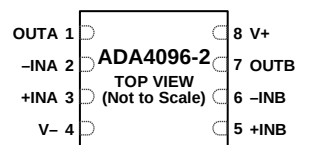
Figure 1. 8-Lead, MSOP (RM-8), ADA4096-2
