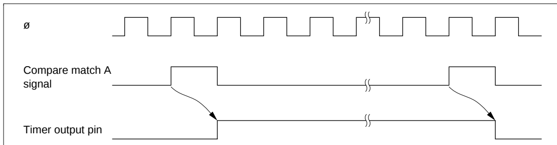
Figure 10-5 Timing of Timer Output
