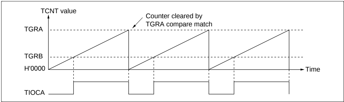
Figure 9-22 Example of PWM Mode Operation (1)
