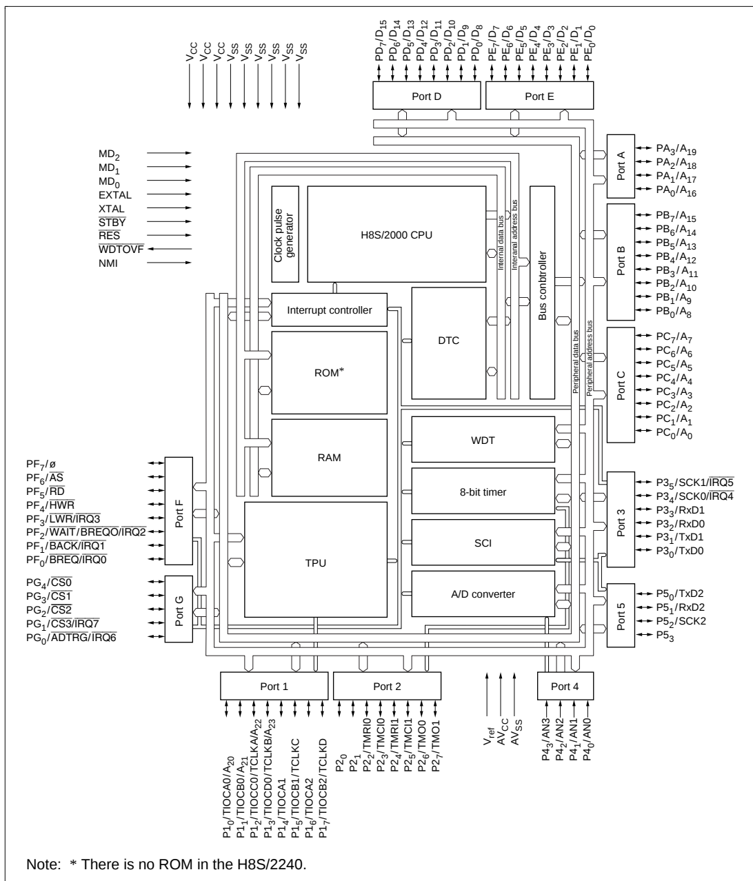
Figure 1-1 Block Diagram
