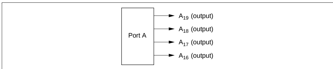
Figure 8-8 Port A Pin Functions (Modes 4 and 5)
