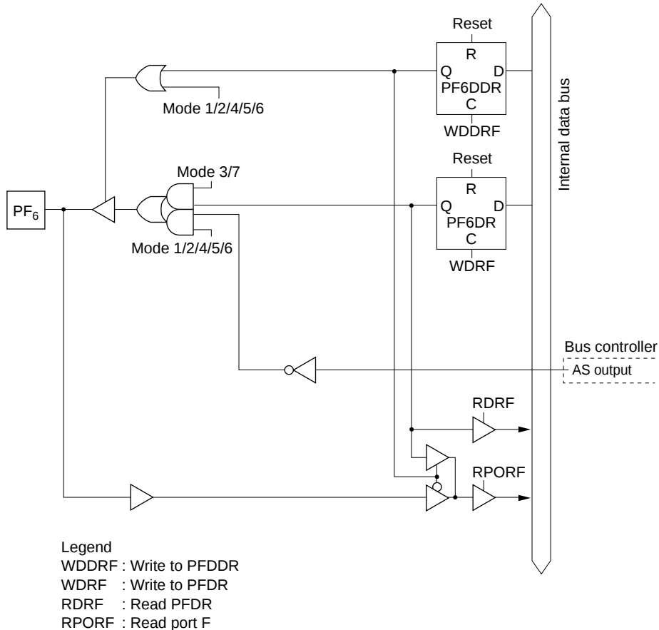
Figure C-11 (g) Port F Block Diagram (Pin PF 6 )
