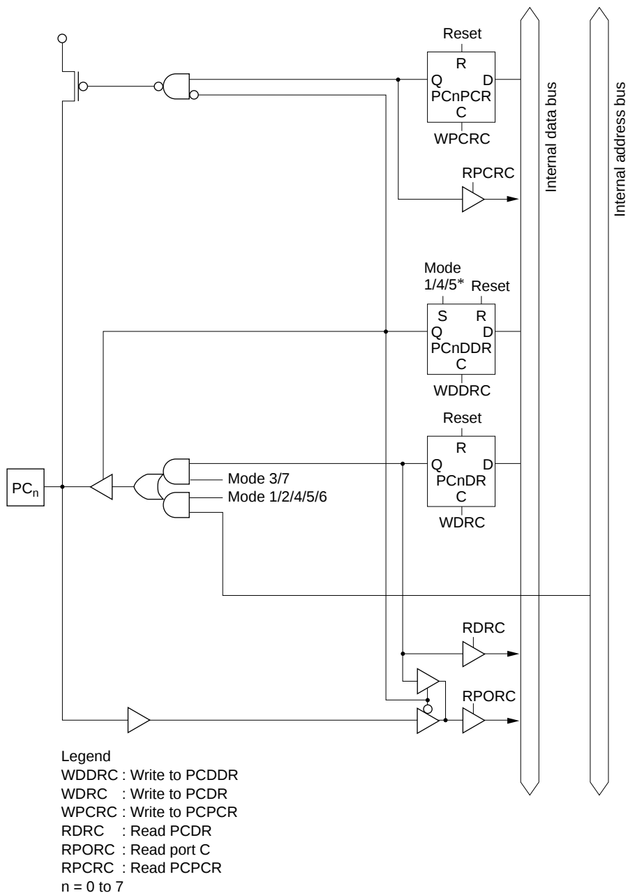
Figure C-8 Port C Block Diagram (Pin PC n )
