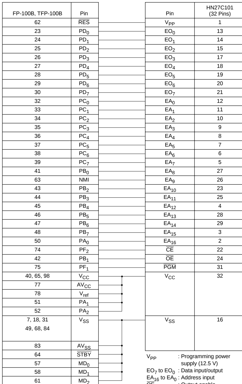
Figure 16-2 Wiring of 100-Pin/32-Pin Socket Adapter
