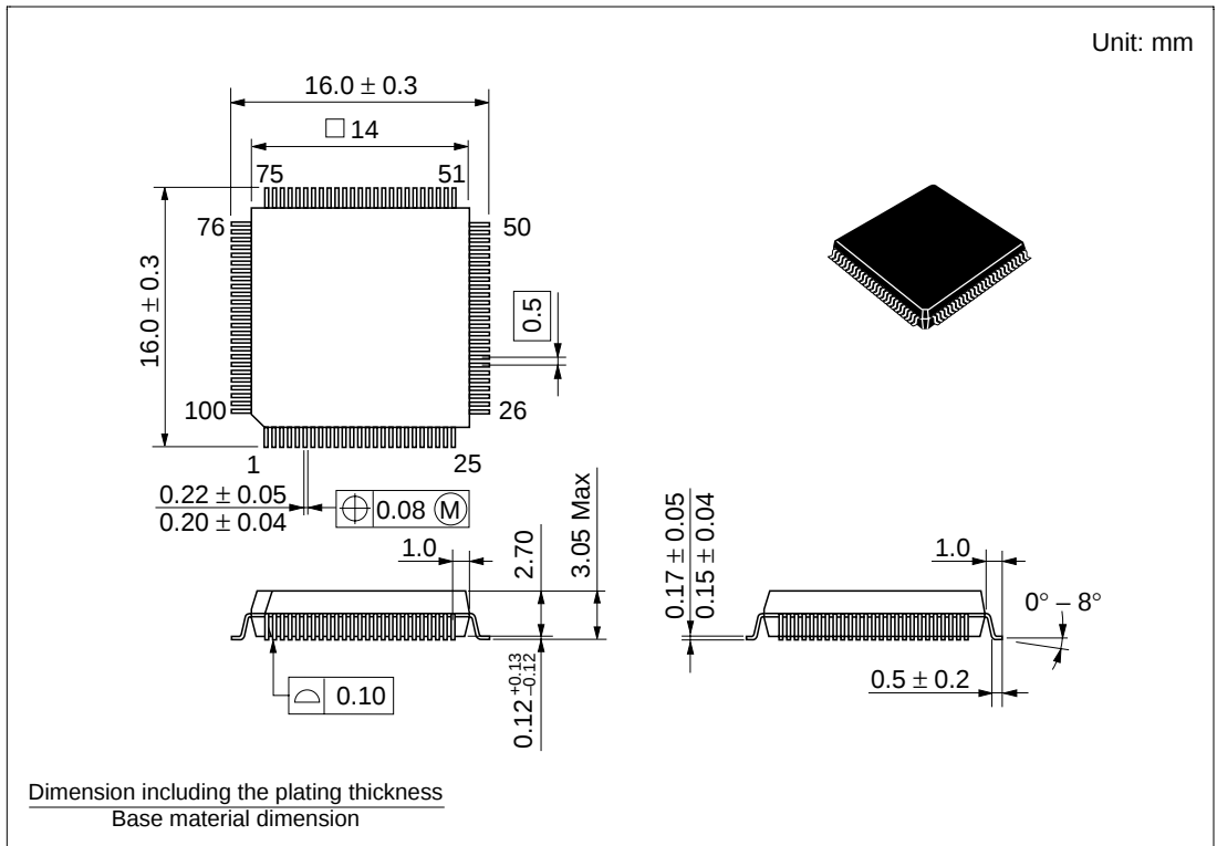
Figure H-1 FP-100B Package Dimensions
