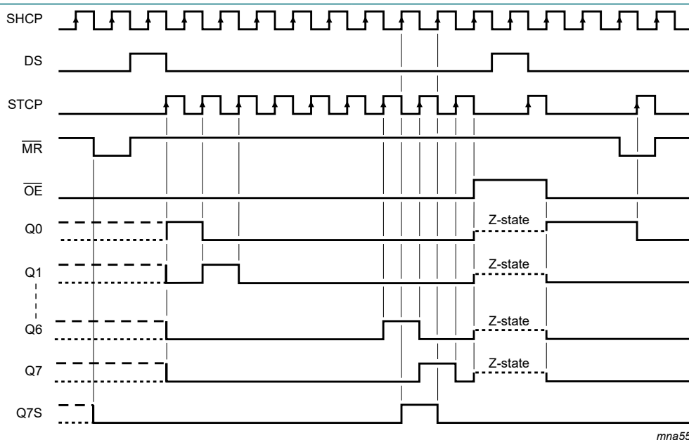
Fig. 5. Timing diagram
